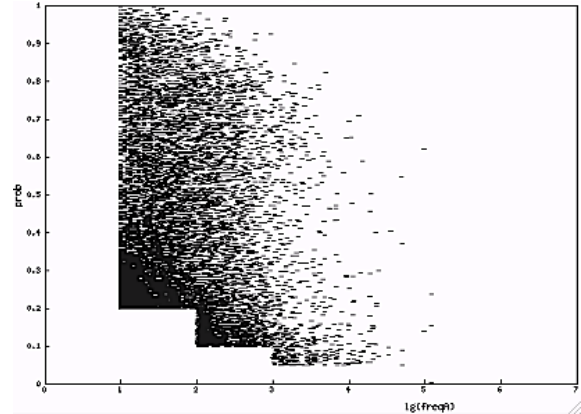
Figure 1: The customized dictionary: the distribution of the Lithuanian-Hungarian translation candidates. Logarithmic frequency of the source words on the x -axis, translation probability on the y -axis.
